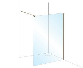
- Corner Panel (in Alcove) - Low Level Brace kit
