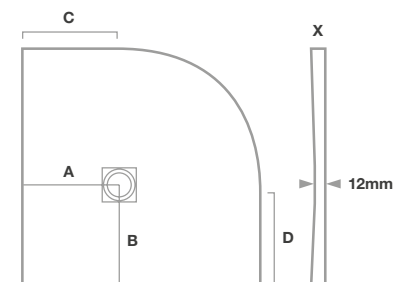
Left Hand Quadrant Offset Shower Tray
